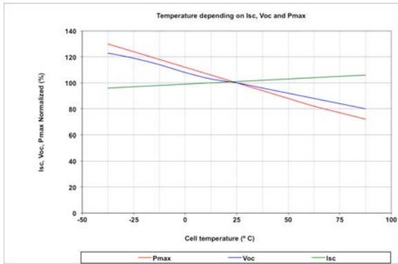
TEMPERATURE
