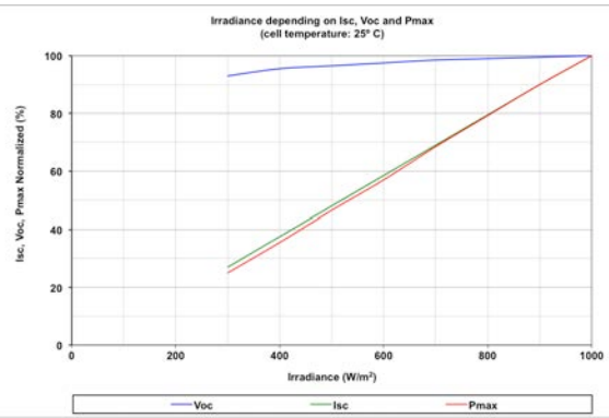
IRRADIANCE
