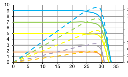
ভোল্টেজ (V) ভোল্টেজ (V) --- I-V 1000 W/m2 --- P-I 1000 W/m2 I-V (-25°C) I-V (0°C) I-V (+25°C) I-V (+50°C) I-V (+75°C) --- I-V 800 W/m2 --- P-I 800 W/m2 --- I-V 600 W/m2 --- P-I 600 W/m2 --- I-V 400 W/m2 --- P-I 400 W/m2 --- I-V 200 W/m2 --- P-I 200 W/m2
